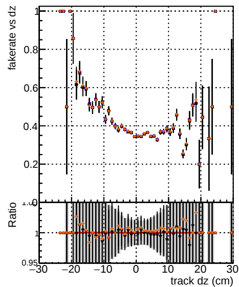
Fake rate vs dz DGM original_lowpt DGM lowpt DGM lowpt_less DGM newbranch_lowpt_less
