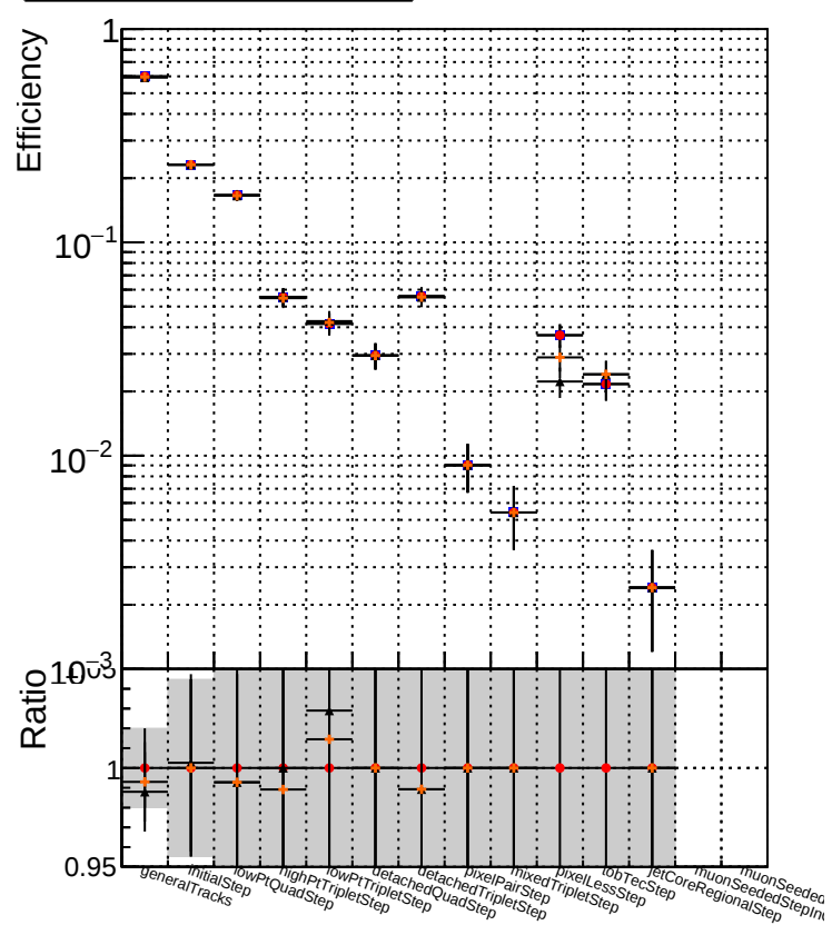
DQM_TT_original_lowpt DQM_TT_newbranch_lowpt DQM_TT_original_lowpt_pLess DQM_TT_newbranch_lowpt_pLess
