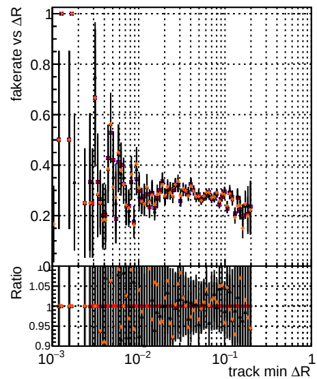
Fake rate vs \Delta R (track, jet) Legend: \Delta R (black dots) \Delta R (red dots) \Delta R (blue dots) \Delta R (orange dots) \Delta R (black dots) \Delta R (red dots) \Delta R (blue dots) \Delta R (orange dots)
