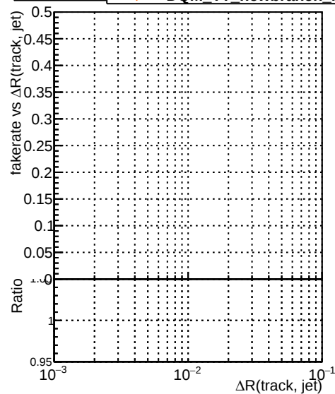
Fake rate vs \Delta R (track, jet) Legend: \Delta R (black dots) \Delta R (red dots) \Delta R (blue dots) \Delta R (orange dots) \Delta R (black dots) \Delta R (red dots) \Delta R (blue dots) \Delta R (orange dots)
