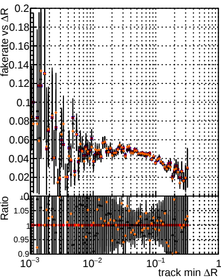
Legend: \Delta R original lowpt \Delta R newbranch lowpt \Delta R original lowpt pLess \Delta R newbranch lowpt pLess
