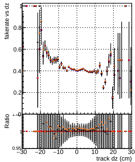
Fake rate vs dz —●— DOM —●— original_lowpt —●— DOM —●— newbranch_lowpt —●— DOM —●— newbranch_lowpt_less
