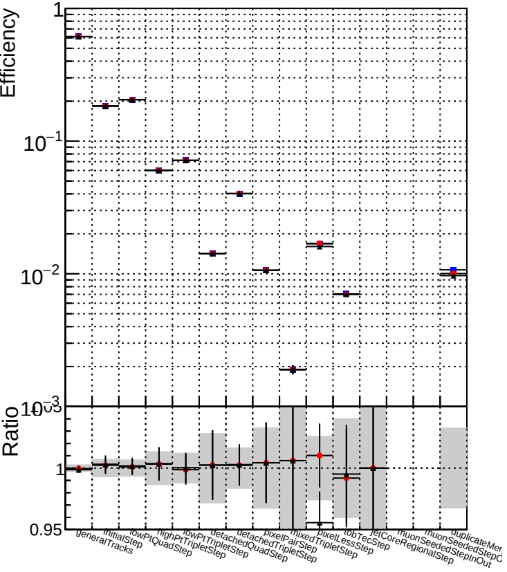
DQM_TT_original DQM_TT_newbranch_pLess DQM_TT_newbranch_pLessMVACand
