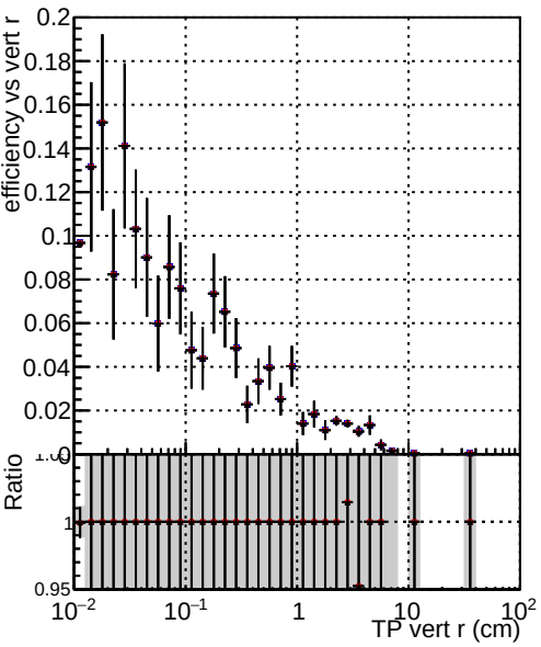
Efficiency vs TP vert r (cm) DQM_TT_original DQM_TT_newbranch_pLess DQM_TT_newbranch_pLessMVACand
