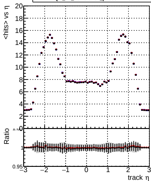
mean hits — DQM_TT_original — DQM_TT_newbranch_pLess — DQM_TT_newbranch_pLessMVACand
