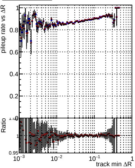
Legend: DQM_TT_original (black), DQM_TT_newbranch_pLess (red), DQM_TT_newbranch_pLessMVACand (blue)
