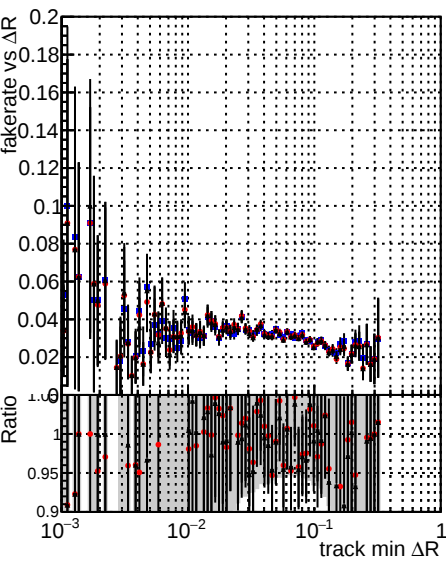
Legend: DQM_TT_original (black), DQM_TT_newbranch_pLess (red), DQM_TT_newbranch_pLessMVACand (blue)
