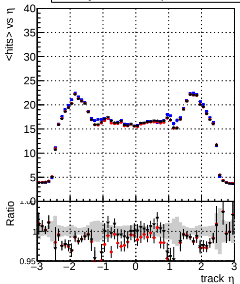
mean hits — DQM_TT_original — DQM_TT_newbranch_pLess — DQM_TT_newbranch_pLessMVACand
