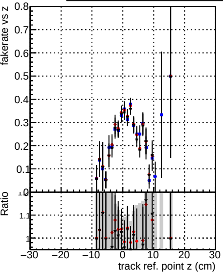
Fake rate vs vertpos —•— DQM TT original —•— DQM TT newbranch_pLess —•— DQM TT newbranch_pLessMVACand
