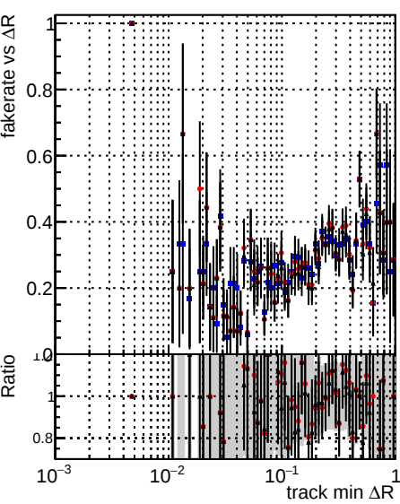
Fake rate vs ΔR(track, jet) Legend: DQM TT original (blue circles) DQM TT newbranch_pLess (red circles) DQM TT newbranch_pLessMVACand (black circles)
