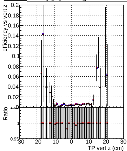
Efficiency vs vert z —●— DQM_TT_original —●— DQM_TT_newbranch_pLess —●— DQM_TT_newbranch_pLessMVACand
