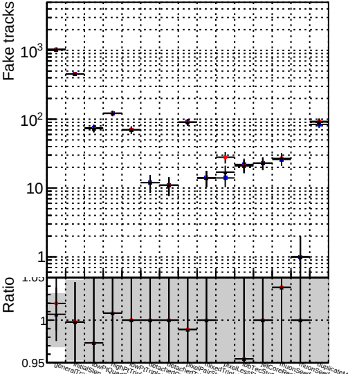
Number DQM_TT_original DQM_TT_newbranch_pLess DQM_TT_newbranch_pLessMVACand
