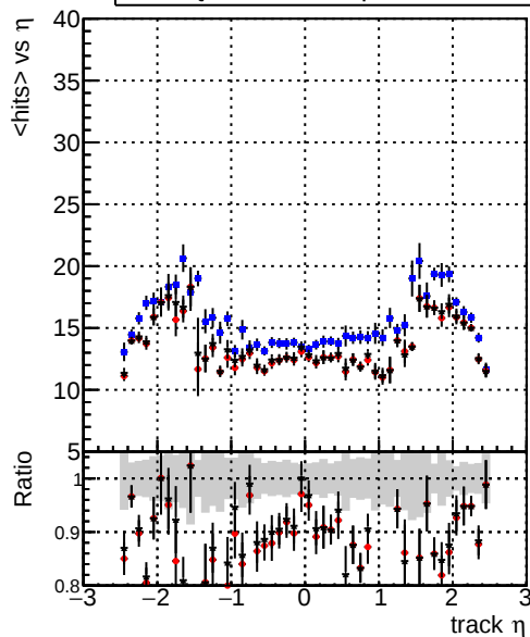
mean hits Legend: DQM_TT_original (blue line) DQM_TT_newbranch_pLess (red line) DQM_TT_newbranch_pLessMVACand (black line)
