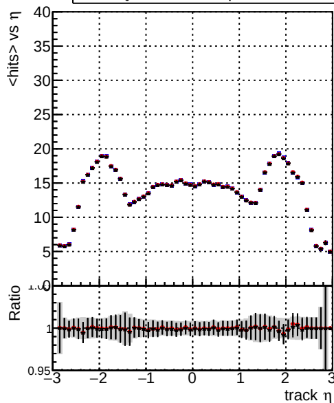
mean hit — DQM_TT_original — DQM_TT_newbranch_pLess — DQM_TT_newbranch_pLessMVACand
