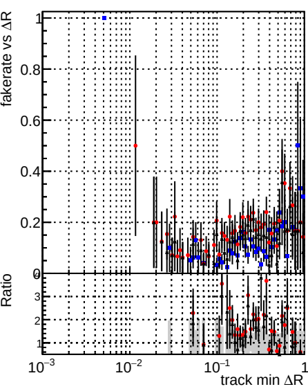
Fake rate vs \Delta R(\text{track, jet}) Legend: \Delta R(\text{track, jet}) (blue dots) \Delta R(\text{track, jet}) (red dots) \Delta R(\text{track, jet}) (black dots)
