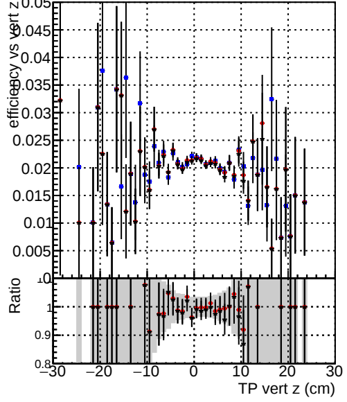
Efficiency vs TP vert z —●— DQM_TT_original —●— DQM_TT_newbranch_pLess —●— DQM_TT_newbranch_pLessMVACand
