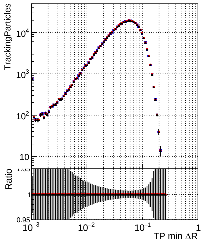
N of simulated tracks ■ DQM TT original ● DQM TT_newbranch_pLess ▲ DQM TT_newbranch_pLessMVACand
