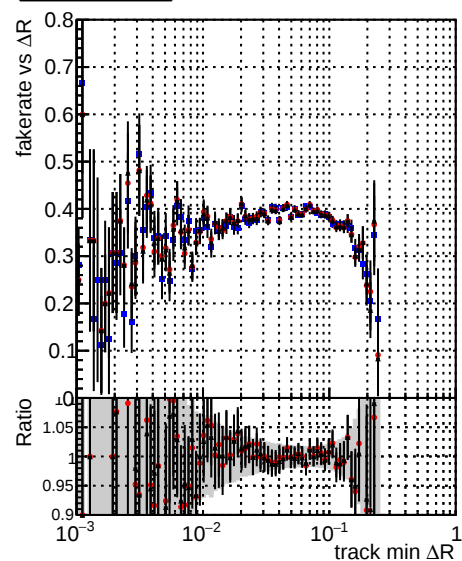
Legend for Fake rate vs \Delta R , Duplicates Rate vs \Delta R , and Pileup rate vs \Delta R : \blacksquare DQM TT original \bullet DQM TT newbranch_pLess \blacktriangledown DQM TT newbranch_pLessMVACand
