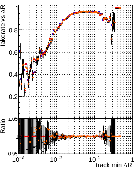
Fake rate vs \Delta R(\text{track, jet}) Legend: original newbranch original pLess newbranch pLess
