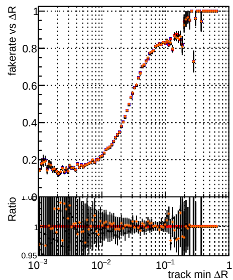
Legend for Fake rate vs \Delta R (track min \Delta R ): tt original (black line) tt newbranch pLess (red line)
