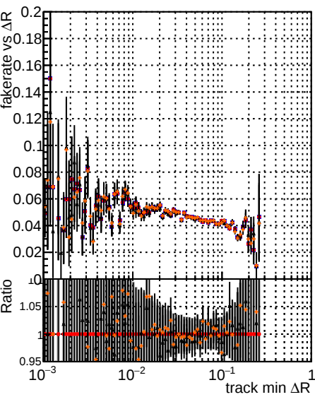
Fake rate vs \Delta R (track, jet) Legend: DOM TT original DOM TT newbranch DOM TT original pLess DOM TT newbranch pLess
