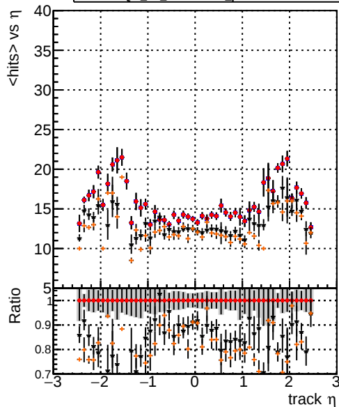
mean hit Legend: DQM_TT_original (blue line), DQM_TT_newbranch (red line), DQM_TT_original_pLess (black line), DQM_TT_newbranch_pLess (orange line)
