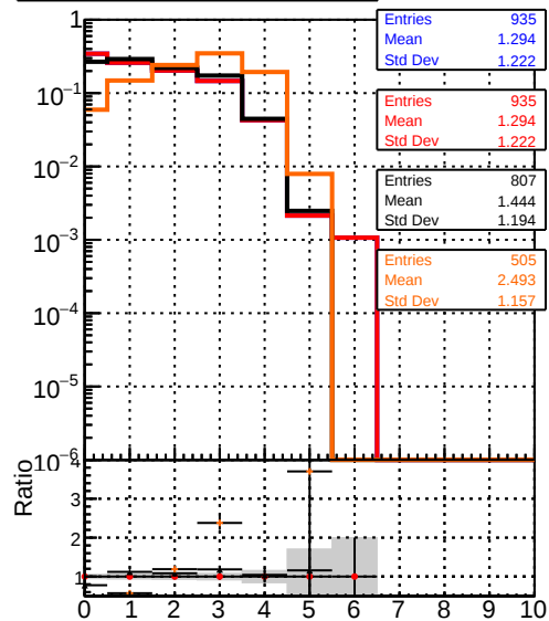
mean hit Legend: DQM_TT_original (blue line), DQM_TT_newbranch (red line), DQM_TT_original_pLess (black line), DQM_TT_newbranch_pLess (orange line)
