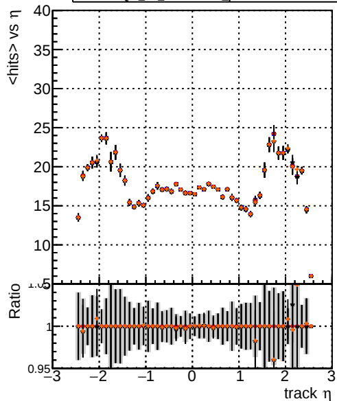
mean hits — DQM_TT_original — DQM_TT_newbranch — DQM_TT_original_pLess — DQM_TT_newbranch_pLess
