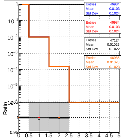
mean hit DQM_TT_original DQM_TT_newbranch DQM_TT_original_pLess DQM_TT_newbranch_pLess
