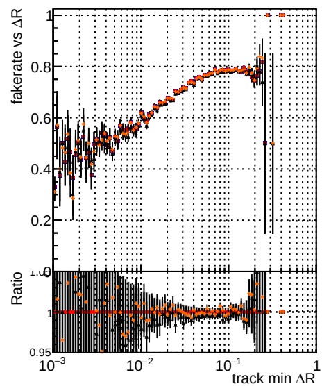
—•— original —•— newbranch —•— original pLess —•— newbranch pLess
