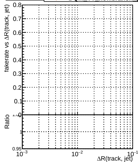
Fake rate vs \Delta R (track, jet) Duplicates Rate vs \Delta R (track, jet) Pileup rate vs \Delta R (track, jet)
