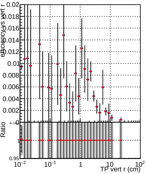
Efficiency vs TP vert r (cm) Legend: 2/CMSSW_12_3_X_2022-02-25-2300/src/DQM_V0001_R0000000001_Global_mkFitOLD_RECO CMSSW_12_3_X_2022-02-25-2300/src/DQM_V0001_R0000000001_Global_mkFitNEW_RECO
