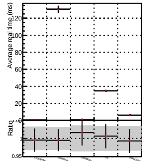
detachedQuadStep
