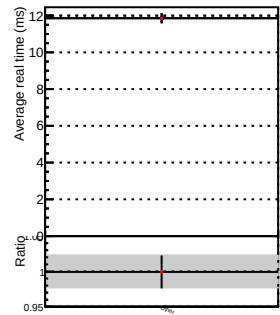
generalTracks
