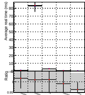
jetCoreRegionalStep
