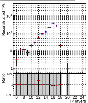
L_R000000001_Global_mkFitNEW_RECO
