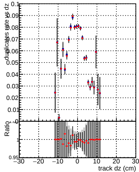
2/CMSSW_12_3_X_2022-02-25-2300/src/DQM_V0001_R0000000001_Global_mkFitOLD_RECO CMSSW_12_3_X_2022-02-25-2300/src/DQM_V0001_R0000000001_Global_mkFitNEW_RECO
