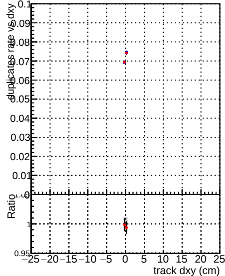
2/CMSSW_12_3_X_2022-02-25-2300/src/DQM_V0001_R0000000001_Global_mkFitOLD_RECO CMSSW_12_3_X_2022-02-25-2300/src/DQM_V0001_R0000000001_Global_mkFitNEW_RECO
