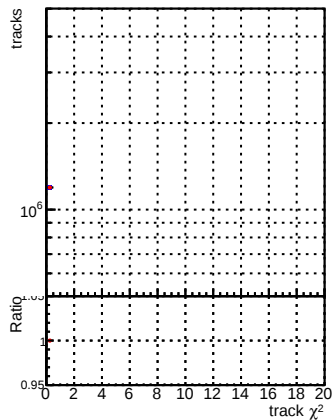
N of reco track vs. \chi^2 — 2/CMSSW_12_3_X_2022-02-25-2300/src/DQM_V0001_R000000001_Global_mkFitOLD_RECO — CMSSW_12_3_X_2022-02-25-2300/src/DQM_V0001_R000000001_Global_mkFitNEW_RECO
