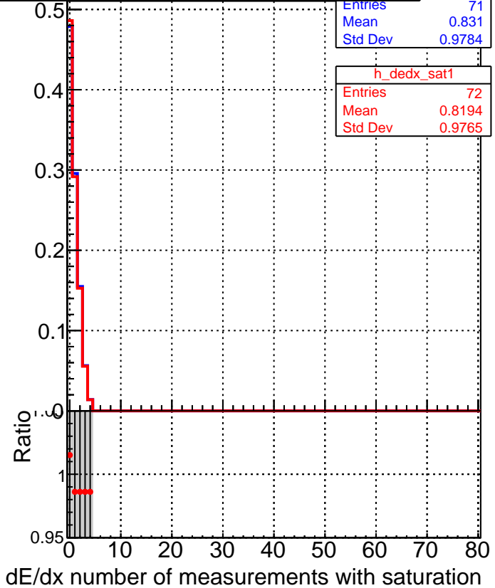
■ 2/CMSSW_12_3_X_2022-02-25-2300/src/DQM_V0001_R000000001_Global_mkFitOLD_RECO ● CMSSW_12_3_X_2022-02-25-2300/src/DQM_V0001_R000000001_Global_mkFitNEW_RECO
