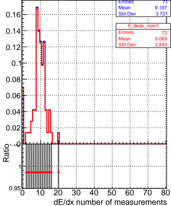
■ 2/CMSSW_12_3_X_2022-02-25-2300/src/DQM_V0001_R000000001_Global_mkFitOLD_RECO ● CMSSW_12_3_X_2022-02-25-2300/src/DQM_V0001_R000000001_Global_mkFitNEW_RECO
