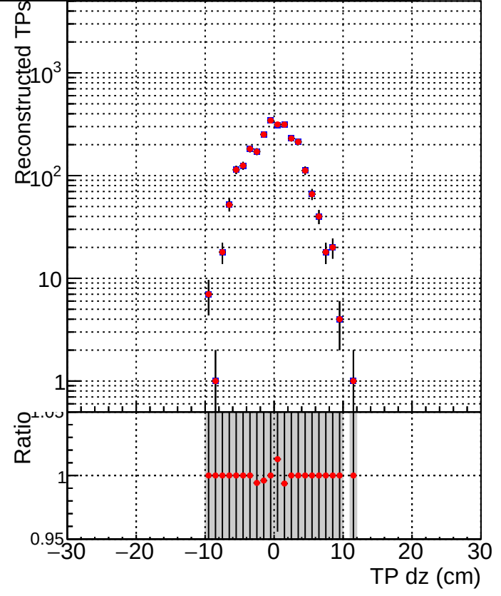
2/CMSSW_12_3_X_2022-02-25-2300/src/DQM_V0001_R0000000001_Global_mkFitOLD_RECO CMSSW_12_3_X_2022-02-25-2300/src/DQM_V0001_R0000000001_Global_mkFitNEW_RECO
