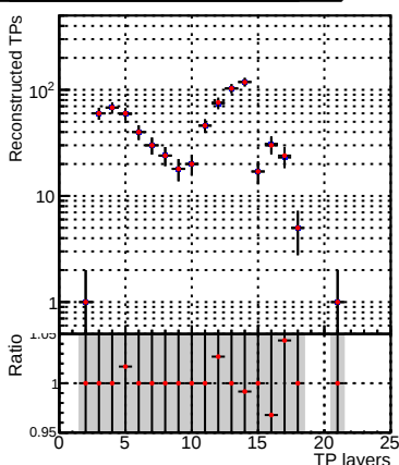
L_R000000001__Global__mkFitNEW__RECO
