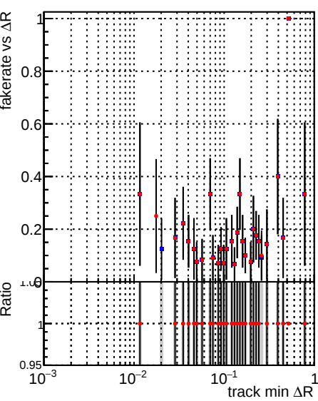
2/CMSSW_12_3_X_2022-02-25-2300/src/DQM_V0001_R000000001_Global_mkFitOLD_RECO Fake rate vs \Delta R(\text{track, jet}) CMSSW_12_3_X_2022-02-25-2300/src/DQM_V0001_R000000001_Global_mkFitNEW_RECO
