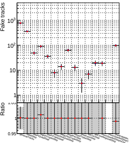
Number CMSSW_12_3_X_2022-02-25-2300/src/DQM_V0001_R000000001_Global_mkFitNEW_RECO
