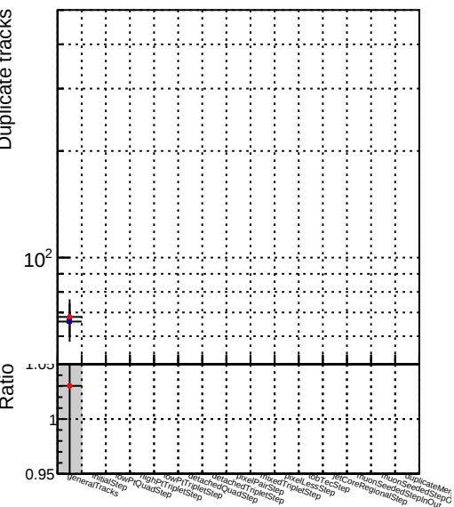
Number CMSSW_12_3_X_2022-02-25-2300/src/DQM_V0001_R000000001_Global_mkFitNEW_RECO
