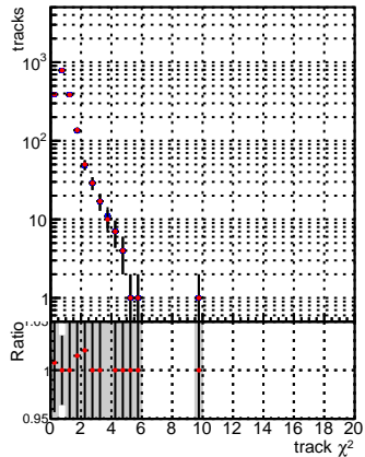
N of reco track vs. \chi^2 for 2/CMSW_12_3_X_2022-02-25-2300/src/DQM_V0001_R0000000001_Global_mkFitOLD_RECO and 2/CMSW_12_3_X_2022-02-25-2300/src/DQM_V0001_R0000000001_Global_mkFitNEW_RECO
