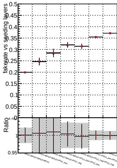
Fake rate vs. 2/CMSSW_12_3_X_2022-02-25-2300/src/DQM_V0001_R000000001_Global_mkFitOLD_RECO CMSSW_12_3_X_2022-02-25-2300/src/DQM_V0001_R000000001_Global_mkFitNEW_RECO
