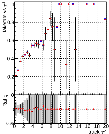
Fake rate vs. 2/CMSSW_12_3_X_2022-02-25-2300/src/DQM_V0001_R000000001_Global_mkFitOLD_RECO CMSSW_12_3_X_2022-02-25-2300/src/DQM_V0001_R000000001_Global_mkFitNEW_RECO
