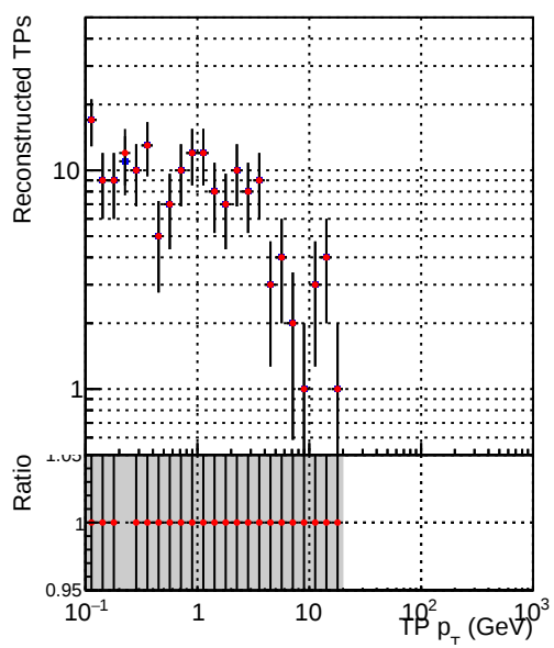
—●— 2/CMSSW_12_3_X_2022-02-25-2300/src/DQM_V0001_R000000001_Global_mkFitOLD_RECO —●— CMSSW_12_3_X_2022-02-25-2300/src/DQM_V0001_R000000001_Global_mkFitNEW_RECO
