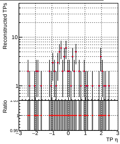
—●— 2/CMSSW_12_3_X_2022-02-25-2300/src/DQM_V0001_R000000001_Global_mkFitOLD_RECO —●— CMSSW_12_3_X_2022-02-25-2300/src/DQM_V0001_R000000001_Global_mkFitNEW_RECO
