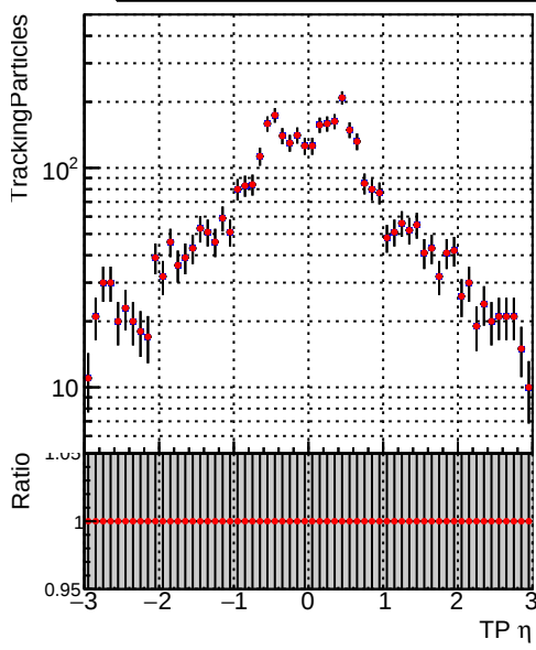
—●— 2/CMSSW_12_3_X_2022-02-25-2300/src/DQM_V0001_R000000001_Global_mkFitOLD_RECO —●— CMSSW_12_3_X_2022-02-25-2300/src/DQM_V0001_R000000001_Global_mkFitNEW_RECO
