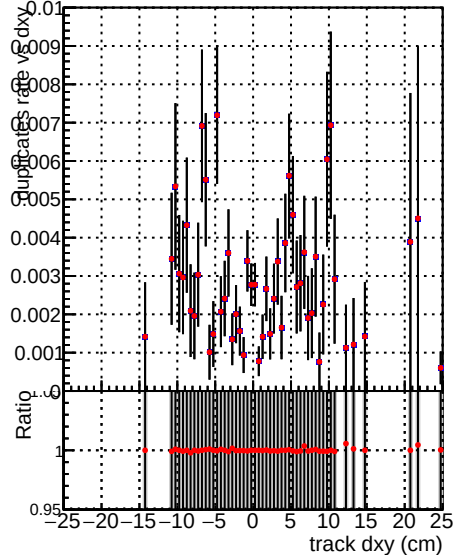
—●— 2/CMSSW_12_3_X_2022-02-25-2300/src/DQM_V0001_R000000001_Global_mkFitOLD_RECO —●— CMSSW_12_3_X_2022-02-25-2300/src/DQM_V0001_R000000001_Global_mkFitNEW_RECO
