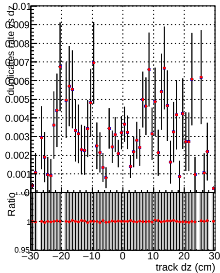
—●— 2/CMSSW_12_3_X_2022-02-25-2300/src/DQM_V0001_R000000001_Global_mkFitOLD_RECO —●— CMSSW_12_3_X_2022-02-25-2300/src/DQM_V0001_R000000001_Global_mkFitNEW_RECO
