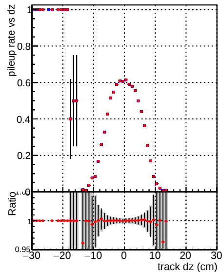
—●— 2/CMSSW 12_3_X 2022-02-25-2300/src/DQM_V0001_R0000000001_Global_mkFitOLD_RECO —●— CMSSW 12_3_X 2022-02-25-2300/src/DQM_V0001_R0000000001_Global_mkFitNEW_RECO
