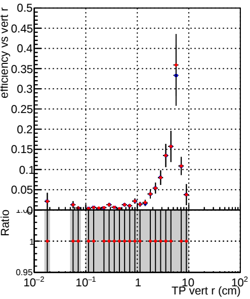
Efficiency vs vertpos Legend: 2/CMSSW_12_3_X_2022-02-25-2300/src/DQM_V0001_R0000000001_Global_mkFitOLD_RECO CMSSW_12_3_X_2022-02-25-2300/src/DQM_V0001_R0000000001_Global_mkFitNEW_RECO
