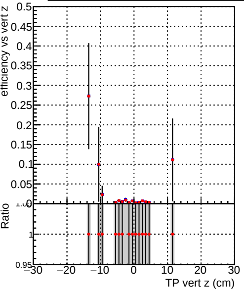
2/CMSSW_12_3_X_2022-02-25-2300/src/DQM_V0001_R0000000001_Global_mkFitOLD_RECO CMSSW_12_3_X_2022-02-25-2300/src/DQM_V0001_R0000000001_Global_mkFitNEW_RECO
