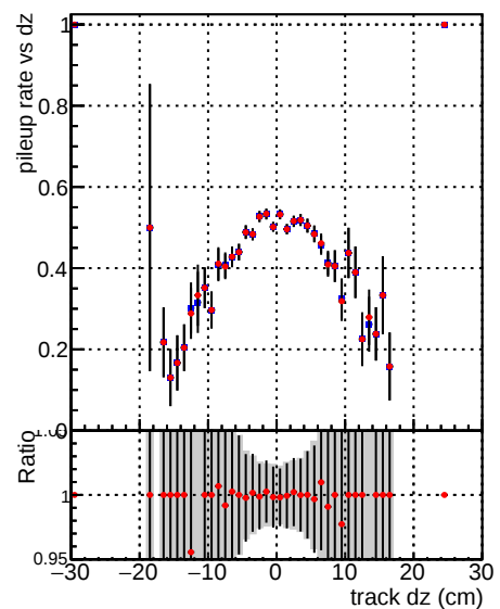
— 2/CMSSW_12_3_X_2022-02-25-2300/src/DQM_V0001_R0000000001_Global_mkFitOLD_RECO — CMSSW_12_3_X_2022-02-25-2300/src/DQM_V0001_R0000000001_Global_mkFitNEW_RECO
