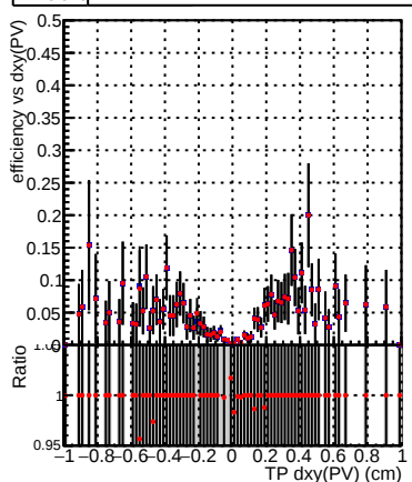
Efficiency — CMSSV
