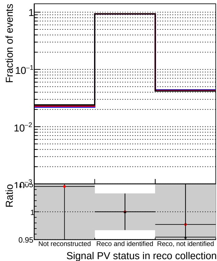
TruePVLocationIndexInRecoVertexCollectionCumulative
