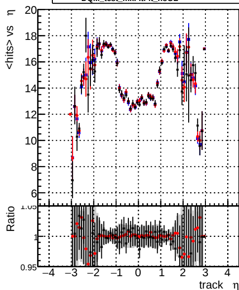
mean hits vs \eta Legend: DQM_test_CKFFitDefault (blue), DQM_test_doubleFit_noOL (red), DQM_test_mkFitFit_noOL (black)
