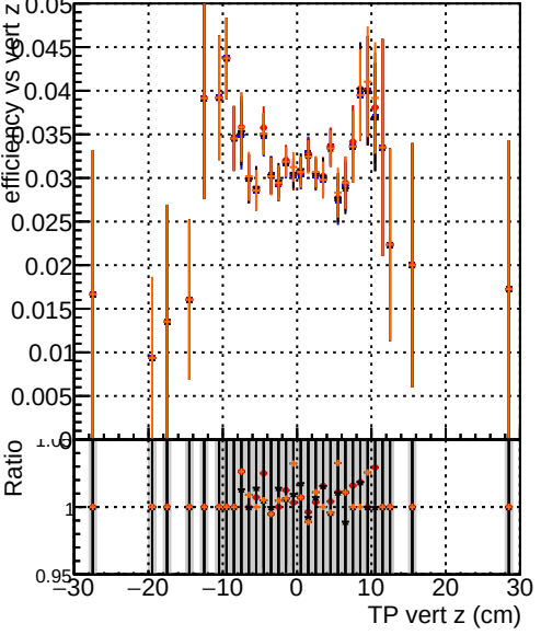
Efficiency vs vertpos Legend: DOM_test_CKFFitDefault DOM_test_mkFitFit DOM_test_mkFitFit_noOL DOM_test_mkFitNOFit_retest
